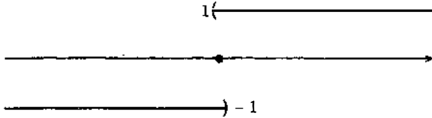
Figure 4.1.2 The signum function
