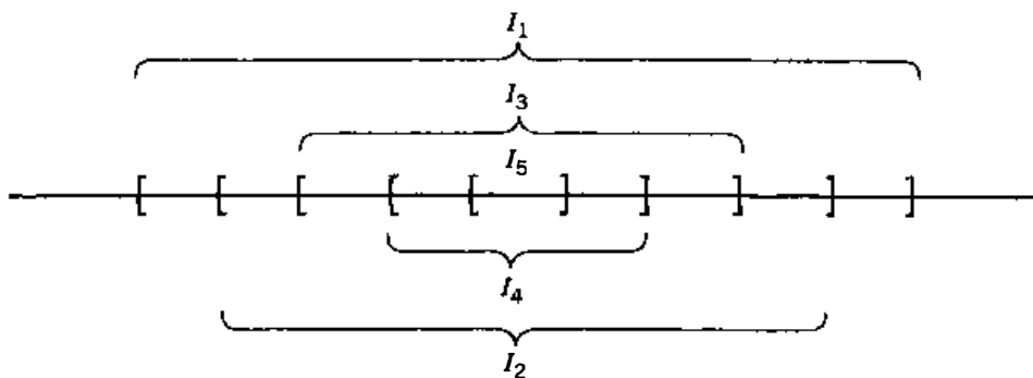
Figure 2.5.1 Nested intervals
