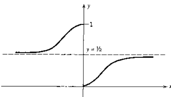
Figure 4.3.2 Graph of h(x) = 1/(e^{1/x} + 1) ( x \neq 0 )
