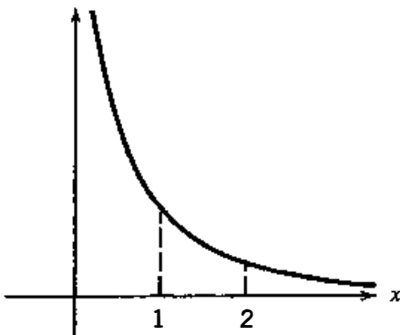
Figure 5.3.1 The function f(x) = 1/x ( x > 0 )
